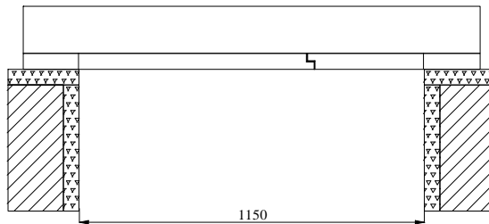
B. Cross section I-I: slab with board insulation material
